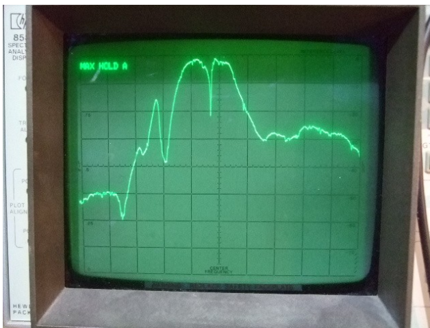
centre=435MHz, 5MHz/div, Gain max= \sim 35dB
