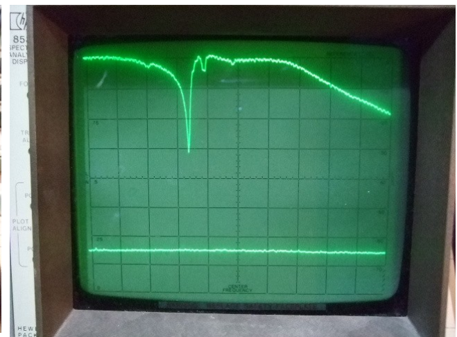
Centre 435MHz; 1MHz/div; gain max= \sim 35dB
